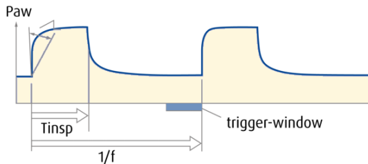
Figure A.2 PCV pressure waveform
