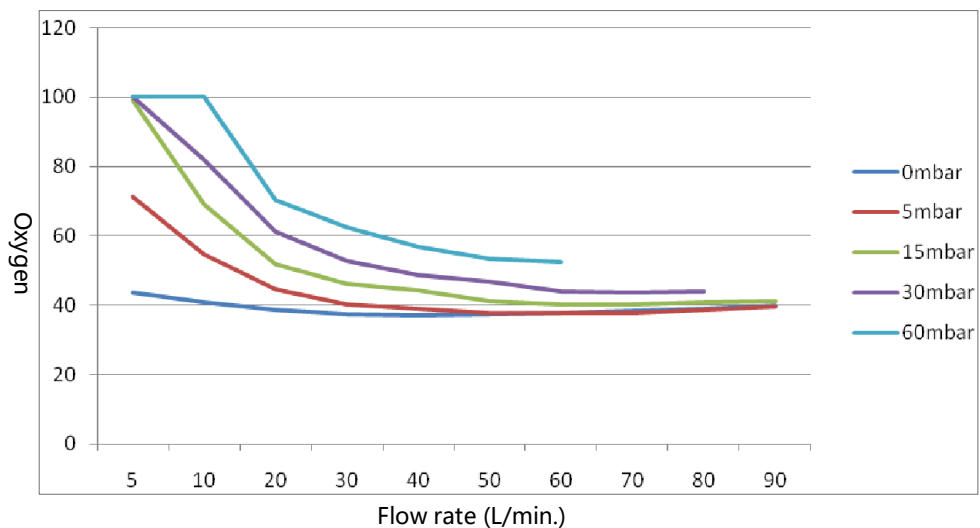
FIGURE 44 Minimum Oxygen Concentration
